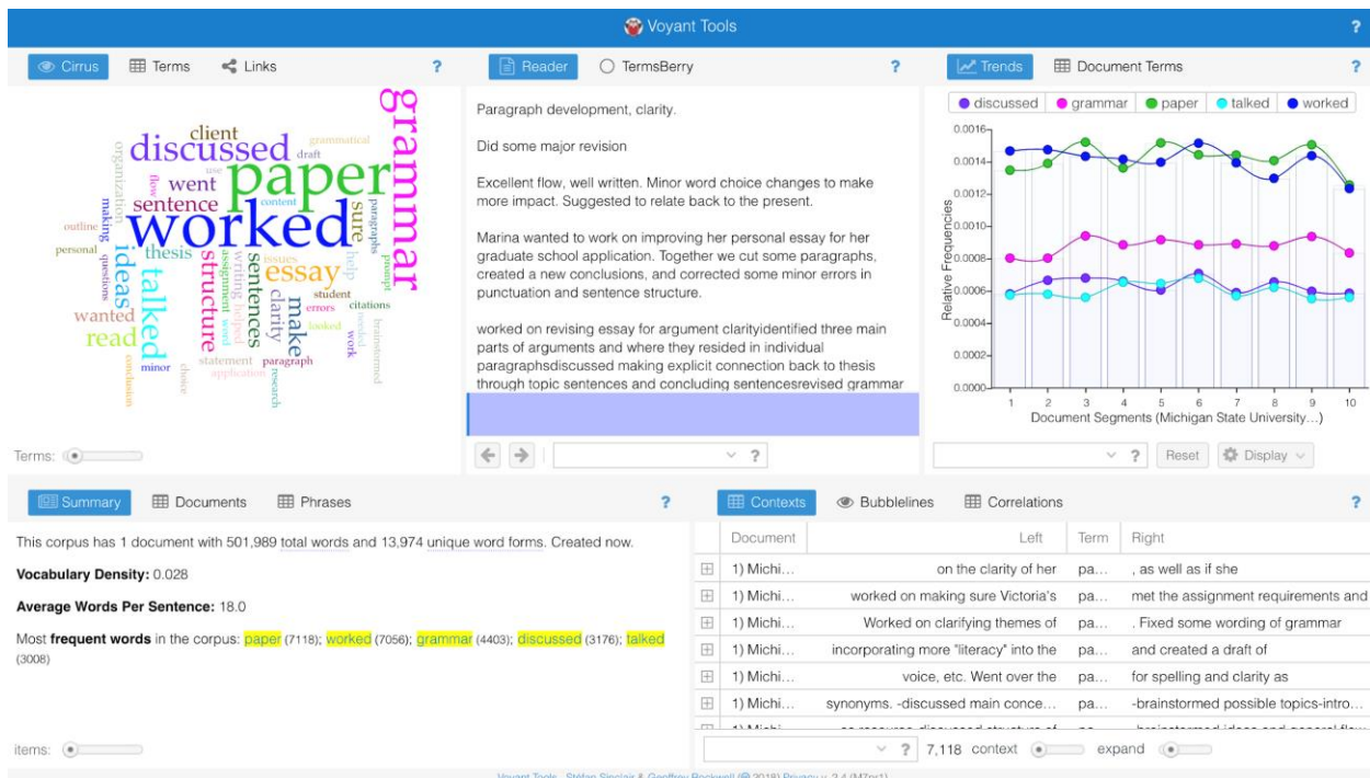
Figure 1. Voyant tools.
